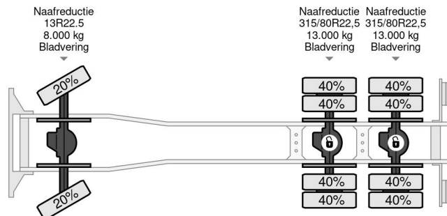
Volvo FL 12.380 6x6 FULL STEEL SUSPENSION MEILLER K... Referentienummer: SN 53819343
