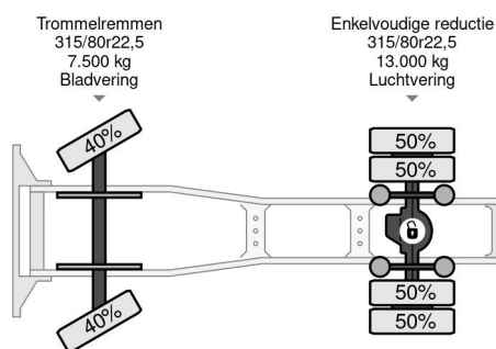
Scania R114-340 LA 4x2 (2 FUEL LINES!!) (EURO 2 / 12 GE...
