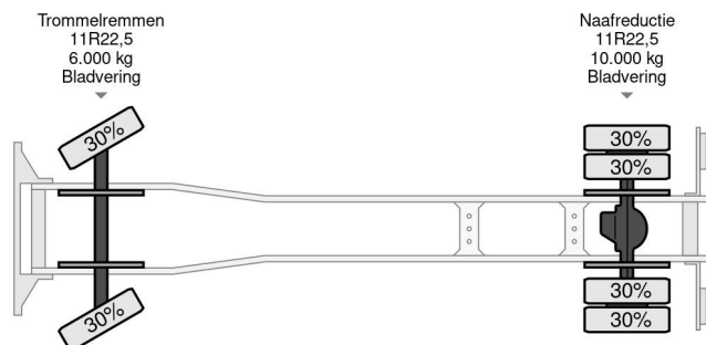
Mercedes-Benz SK 1624 V8 SLEEPERCAB WITH OP... 4x2 Referentienummer: SN 54574025
