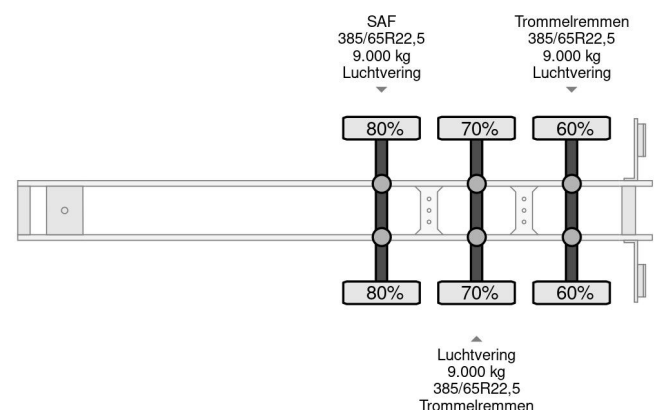
LAG O-3-39 13.60 METER 3-AXLE FLATBED (DRUM BRAK...
