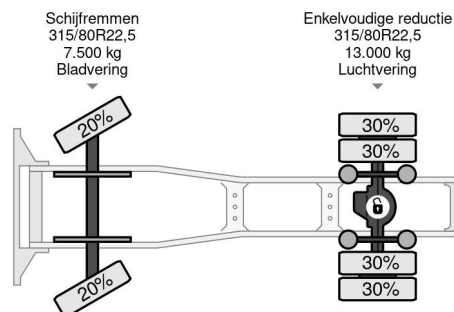
DAF XF 105.460 SPACECAB WITH KIPPER HYDRAUL... 4x2 Referentienummer: SN 54382658 Z
