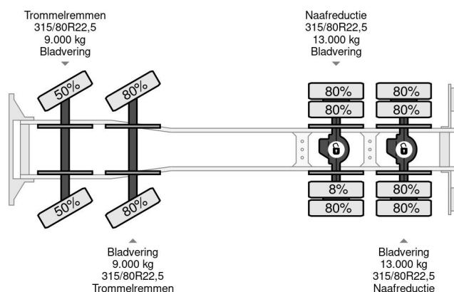
DAF CF 85.430 8x4 FULL STEEL 20m3 KIPPER (EURO 3 / ... Referentienumer: SN 56253918
