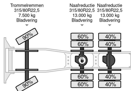
Mercedes-Benz Actros 2640 S 6x4 FULL STEEL TRACTOR ...
