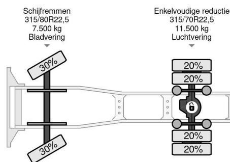
Mercedes-Benz Actros 1843 LS (MP1) (EPS WITH CLU... 4x2
