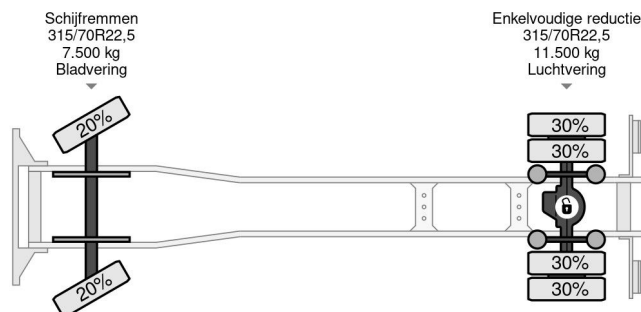
Mercedes-Benz Actros 1840 L (MP1) 4x2 STEEL-AIR SUSP...
