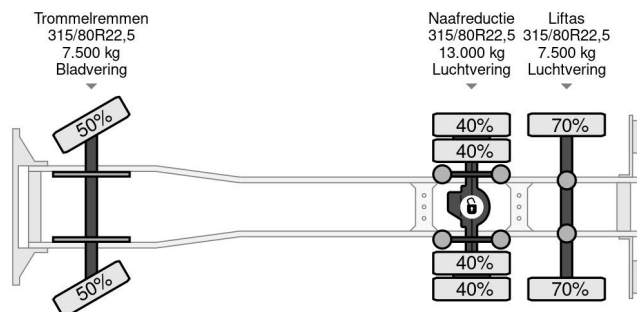
Mercedes-Benz Actros 2540 L 6x2 MP1 WITH V-CRANE & H... Referenznummer: SN 58977623
